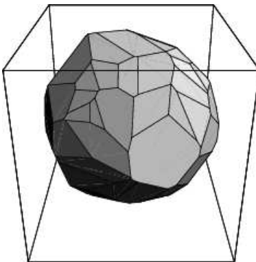
Figure 16: A convex polyhedron P .
